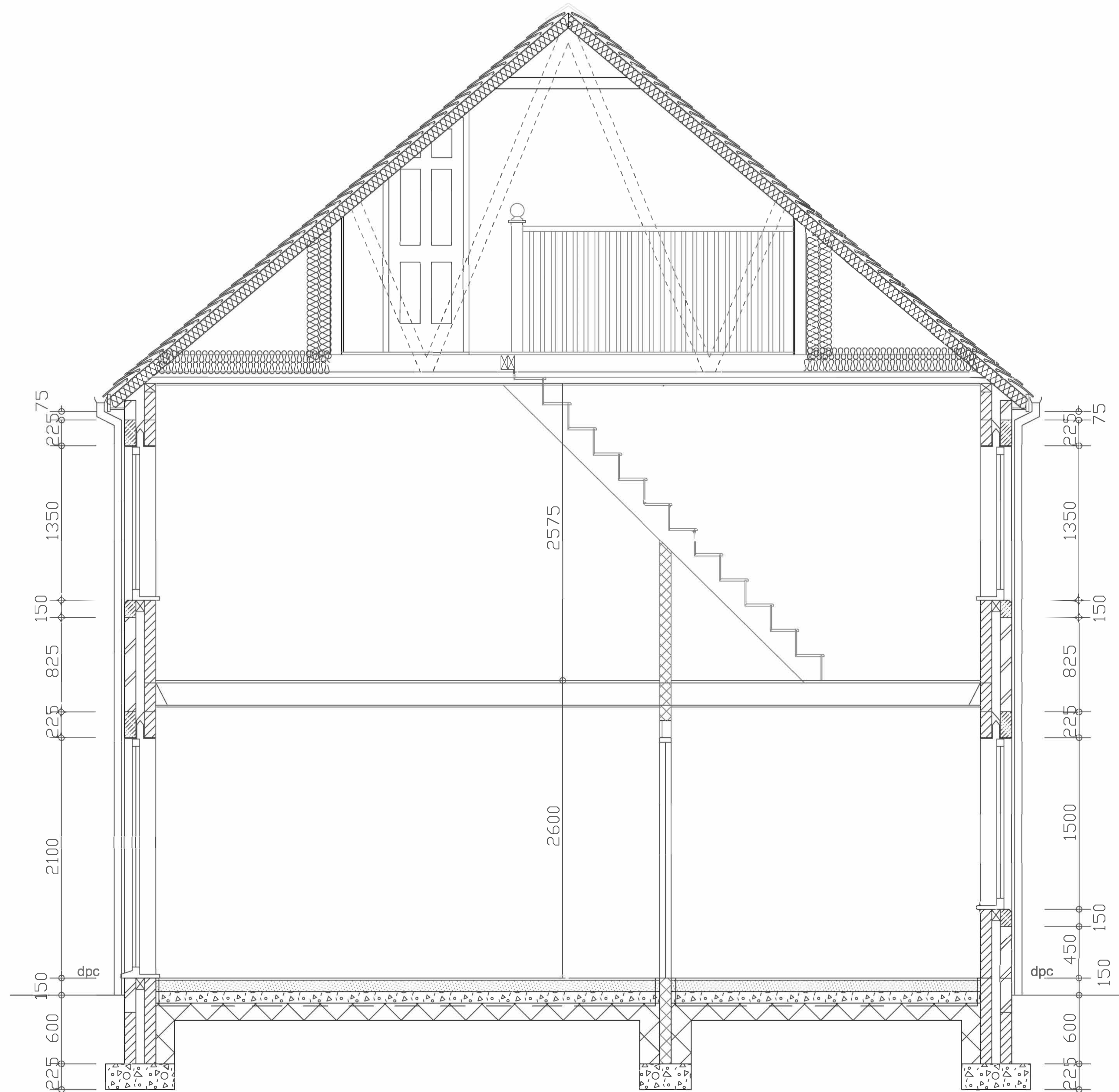
Proposed Section
